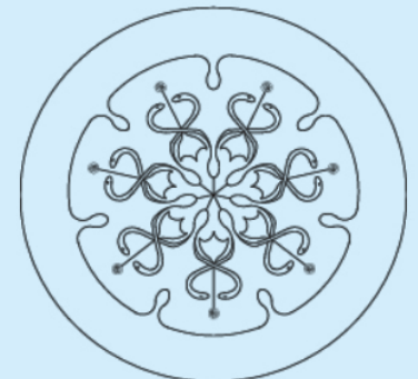
Mercury
